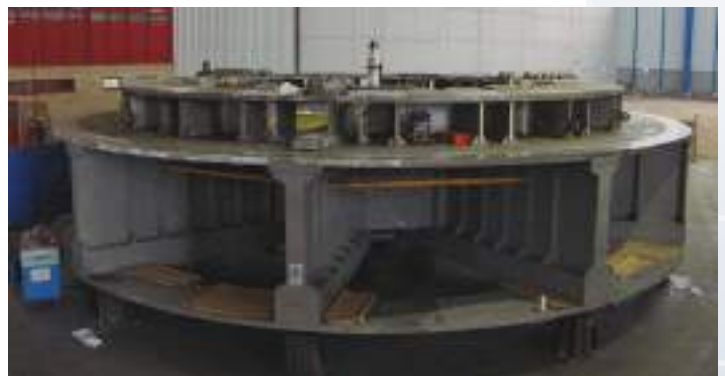
Cryostat Base
