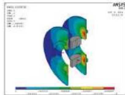
EM simulation of the transient effects on superconducting coils after rapid discharge in a magnetic test bench
