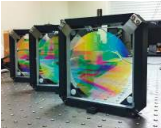
Volume Phase Holographic gratings for ARES spectrograph at Joan Orç telescope(customer IEEC, Barcelona)
