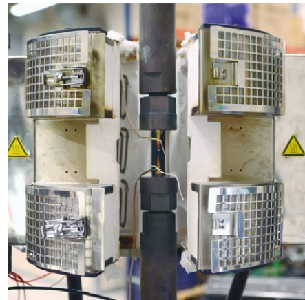
Applus Mechanical Test High Temperature Test Facility
