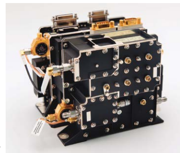
TT&C transponder
