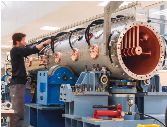
CERN dtl tank
