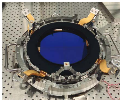
PLATO Focal Plane Assembly CAB_ INTA_LIDAX EM1
