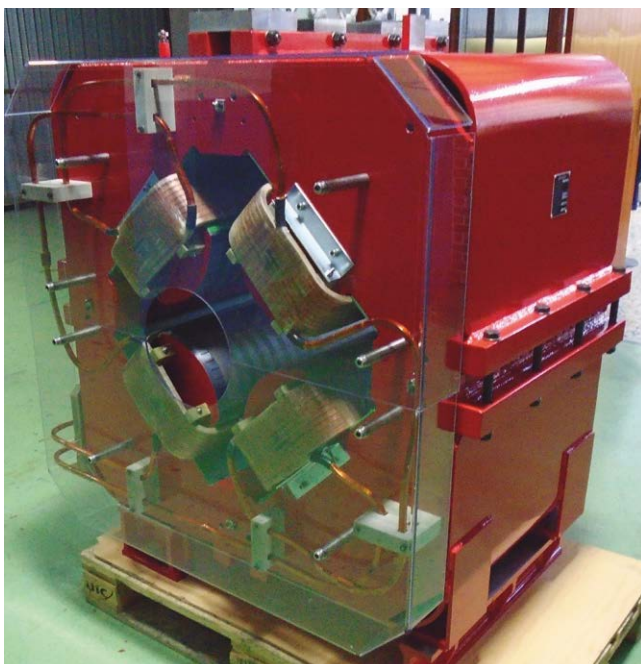
Quadrupole Magnet for the Antiproton Decelerator (AD) - CERN
