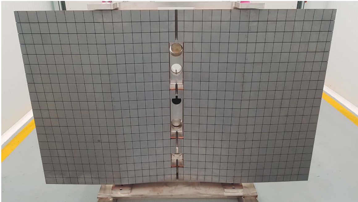
Finished First Wall Panel Semi Prototype
