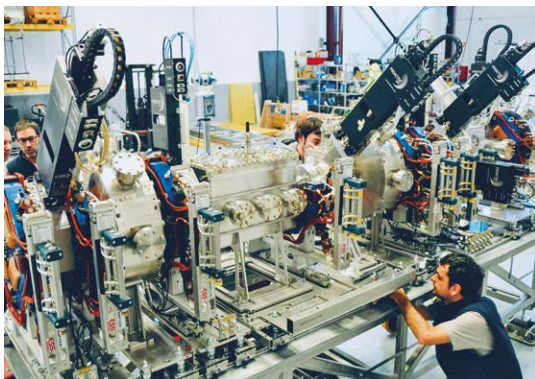
MEFT Assembly at ESS Bilbao premises
