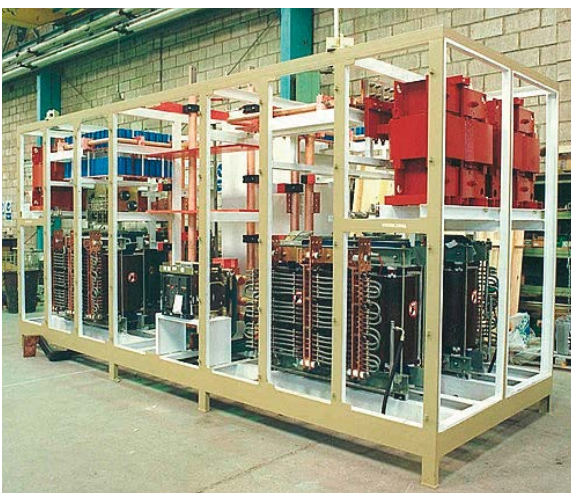
DC Power Supply for CERN
