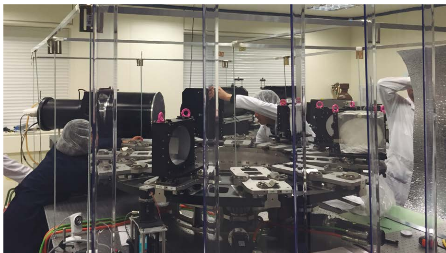
MEGARA spectrograph for the GTC 10m telescope during the assembly at laboratory in Universidad Complutense (customer UCM, Madrid)
