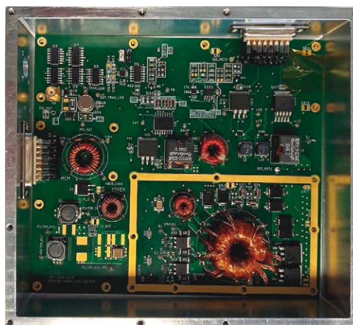
RE_PS Very Low Electromagnetic Noise Power Supply for Scientific Applications
