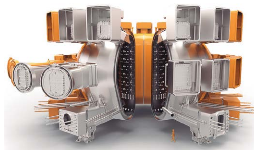
ITER vacuum vessel - (C) ITER Organization - www.iter.org
