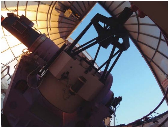
OSN Telescope T90
