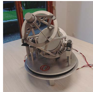
Scaled prototype for testing of control and actuation strategies for the EST main structure
