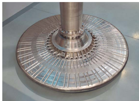
Target Wheel Vessel for European Spallation Source ERIC
