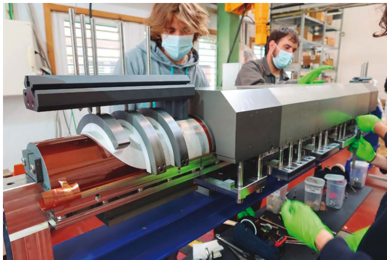
Fabrication of the MCBXFA for the HL-LHC
