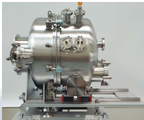
Vacuum Chamber with Temperature Control System from -150° to 200° for CNA
